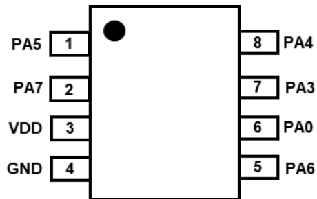
PMS160B-S08B: SOP8 (150mil)
