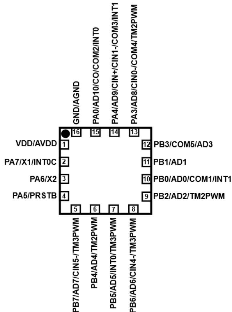
PMS120-1J16A: QFN3*3-16pin (0.5pitch)
