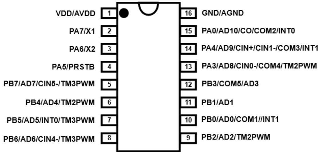
PMS120-S16A: SOP16A (150mil)
