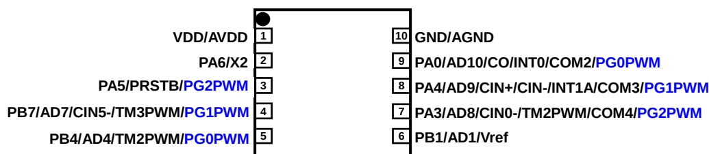
PFS132-4N10 (DFN3*3-10P-0.5pitch)
