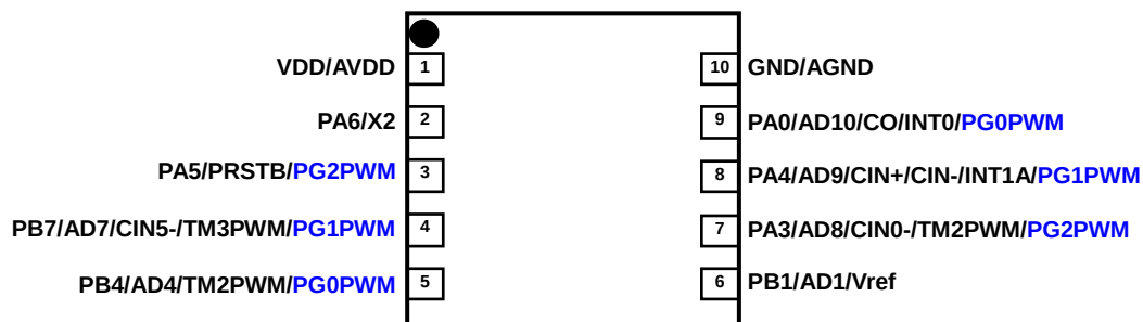
PMS132/PMS132B-4N10 (DFN3*3-10P-0.5pitch)
