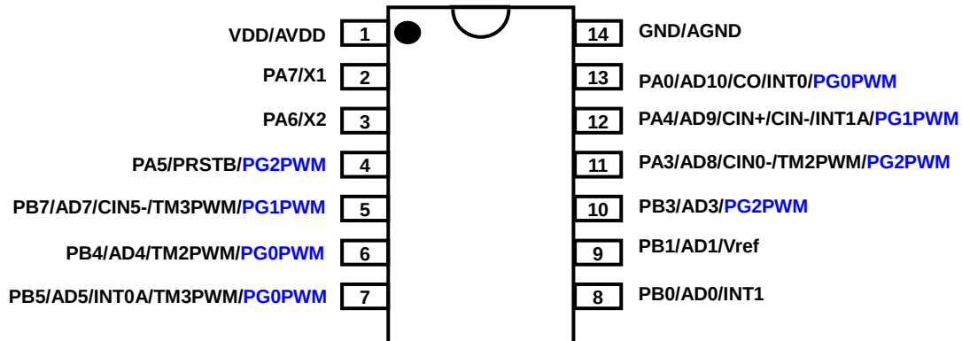
PMS132/PMS132B-S14 (SOP14-150mil)
