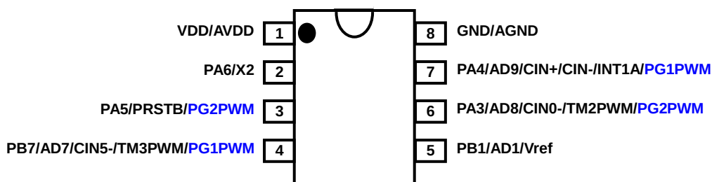
PMS132/PMS132B-S08 (SOP8-150mil)
