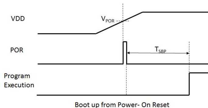
Fig.1: Power-Up Sequence
